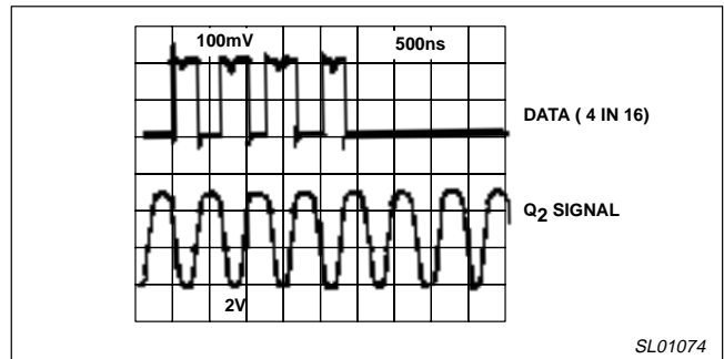
Figure 18. Ringing Circuit Response (4 Data Pulse in 16)
