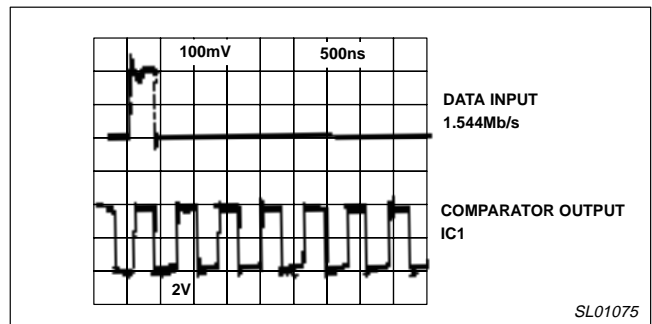
Figure 19. Ringing Circuit to Square Wave Conversion
