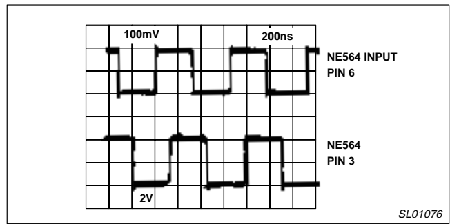
Figure 20. Phase Comparator Signals (in Lock)
